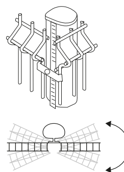
Fence connection at an angle (up to 270°)
